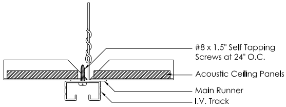
1 Drop Ceiling Grid Installation
