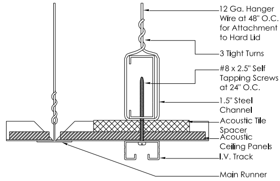
2 Drop Ceiling Grid w/ Channel Backing Installation
