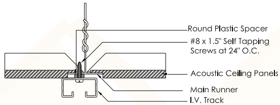
3 Acoustical Tiles w/ Relief Installation
