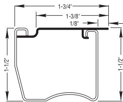
Top Mount
