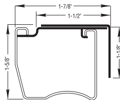
Rear Mount
