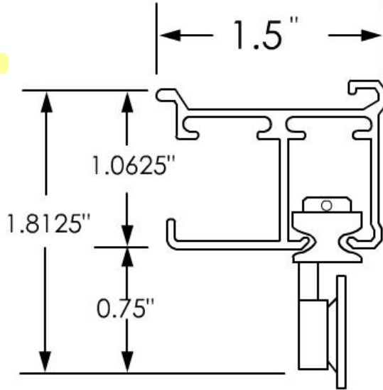
Drapery Track and Carrier
